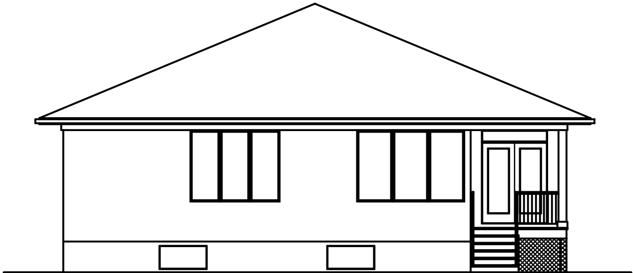
3-1668 REAR ELEVATION SCALE: 1/8"=1'-0"
