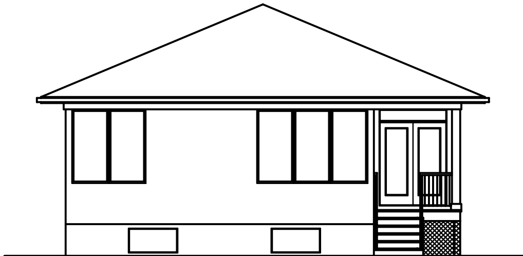
3-1350 REAR ELEVATION SCALE: 1/8"=1'-0"
