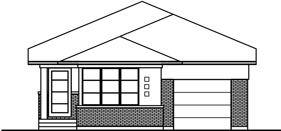
3-1350 FRONT ELEVATION SCALE: 1/8"=1'-0"
